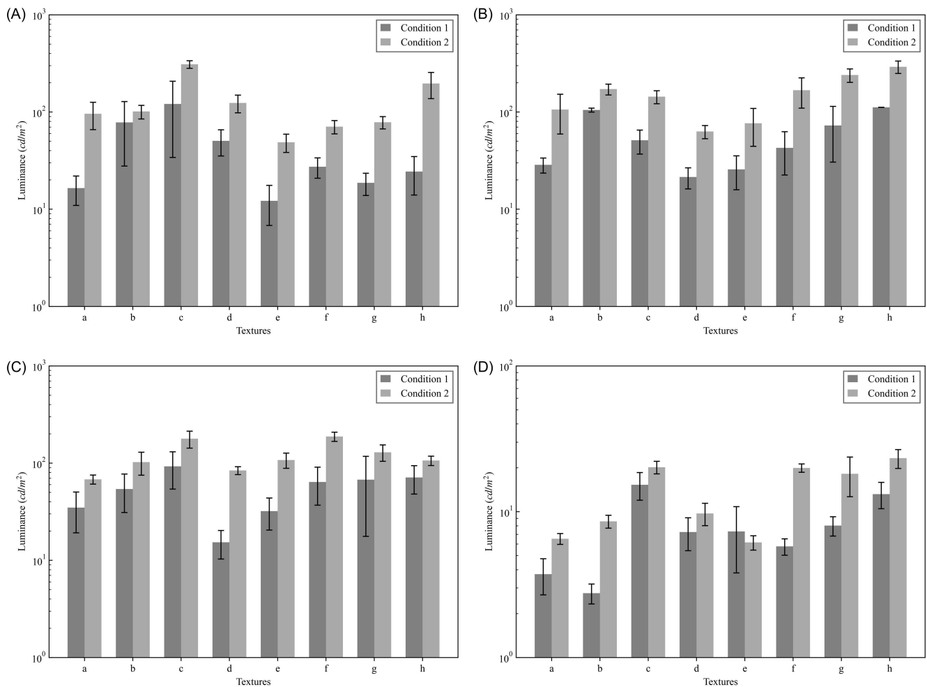
Figure S1. Experimental results. Condition 1 is an illumination stimuli with a mean intensity of 1.0 cd/m 2 , and Condition 2 is 6.0 cd/m 2 .
